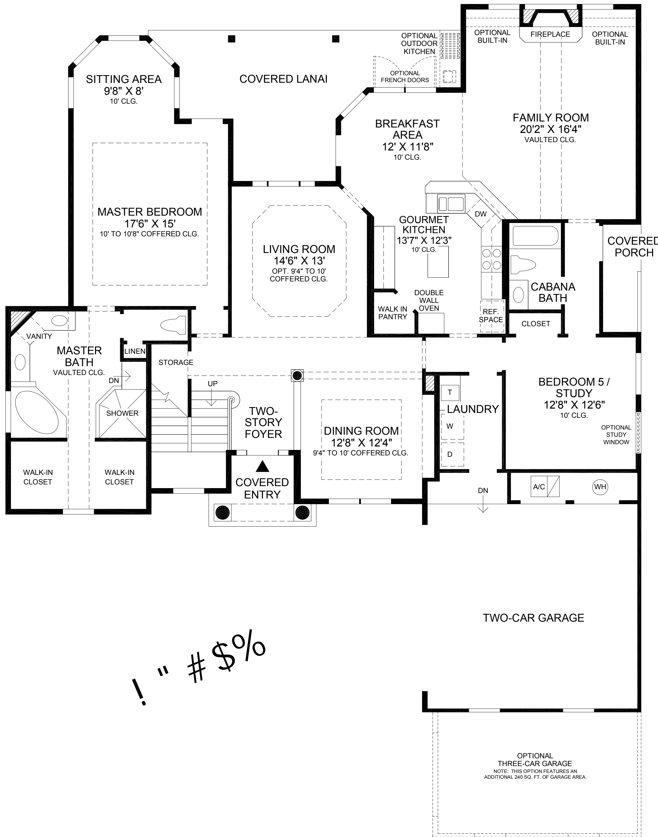
FIRST FLOOR
