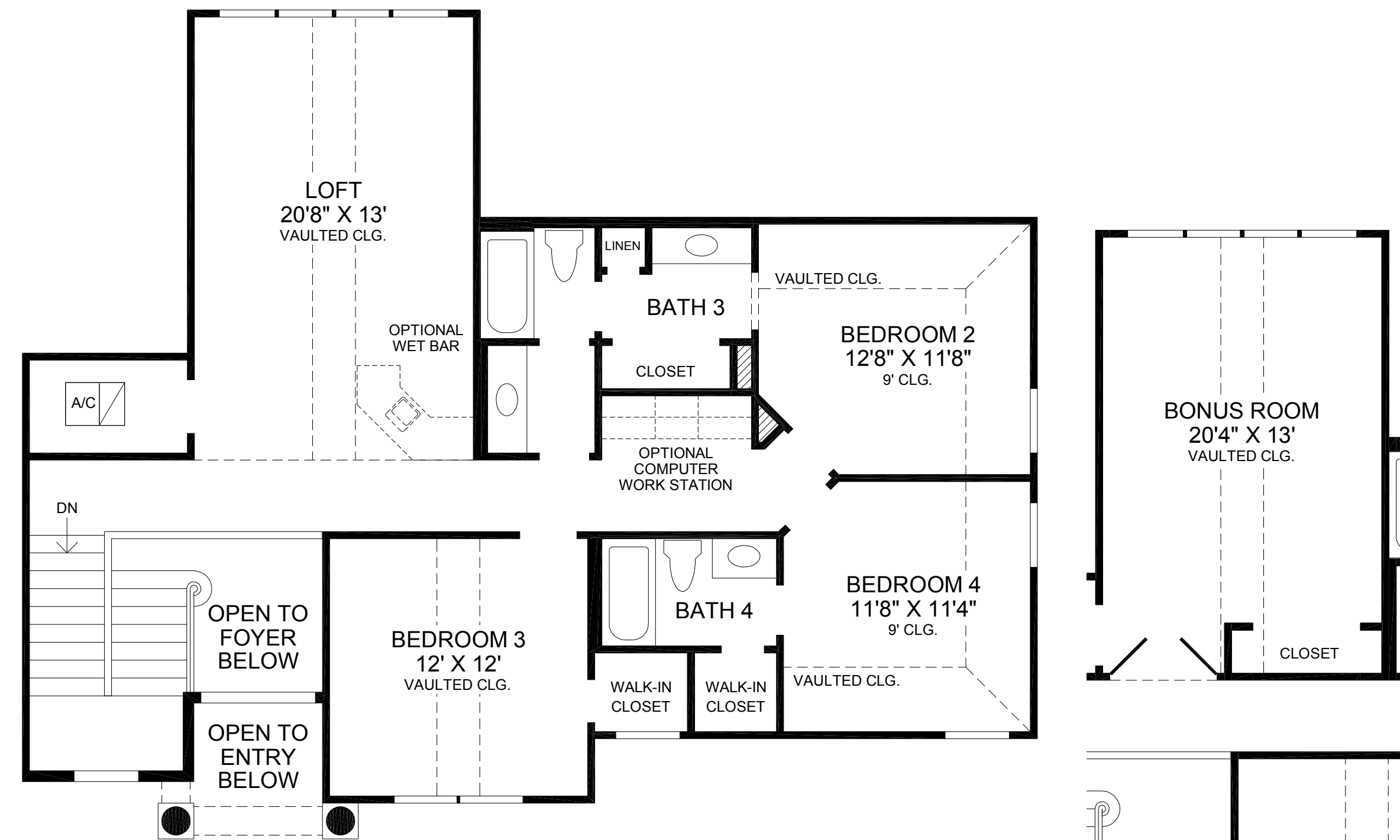
SECOND FLOOR
