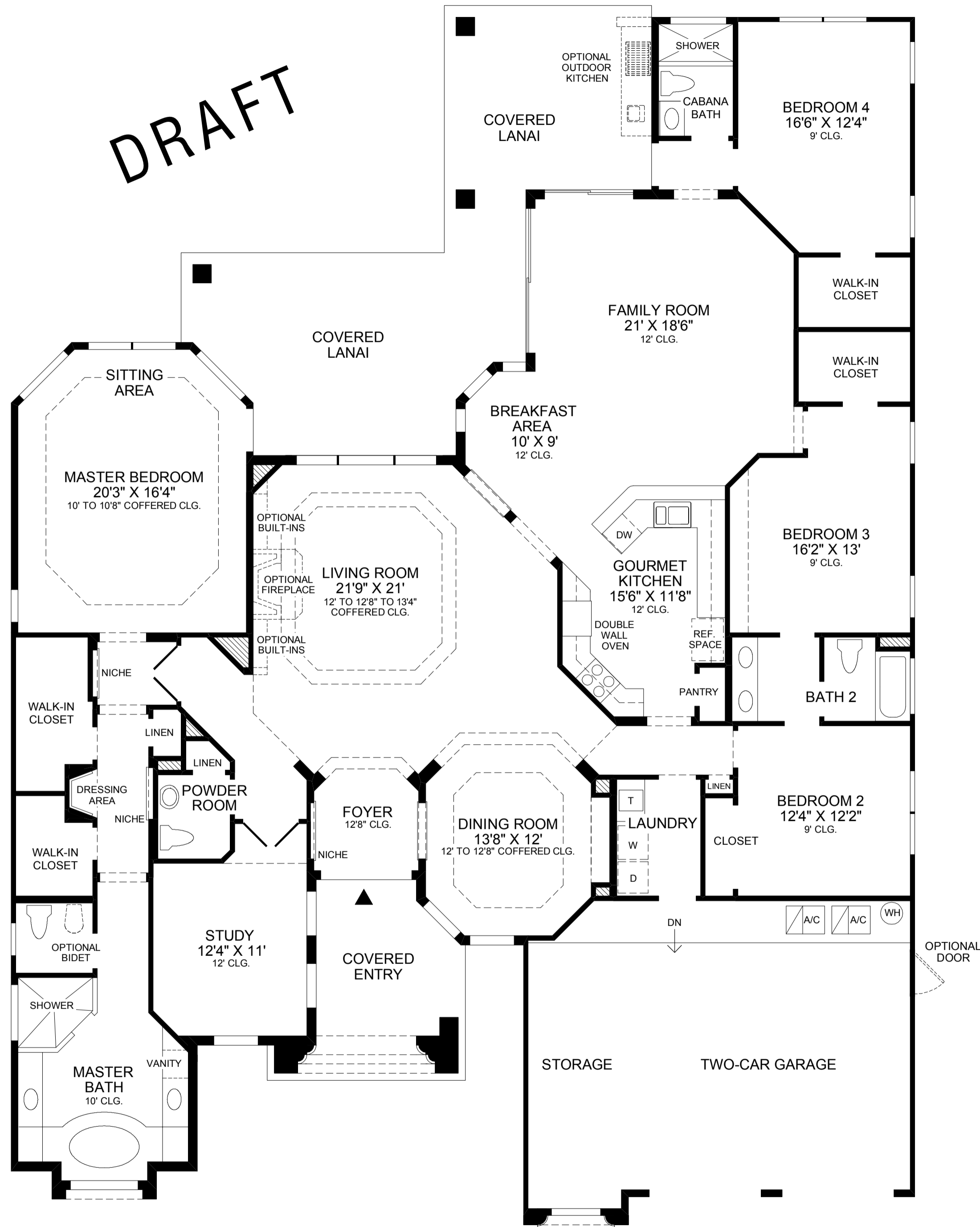
FLOOR PLAN
