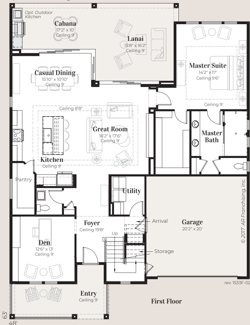
Optional Outdoor Living "A"
