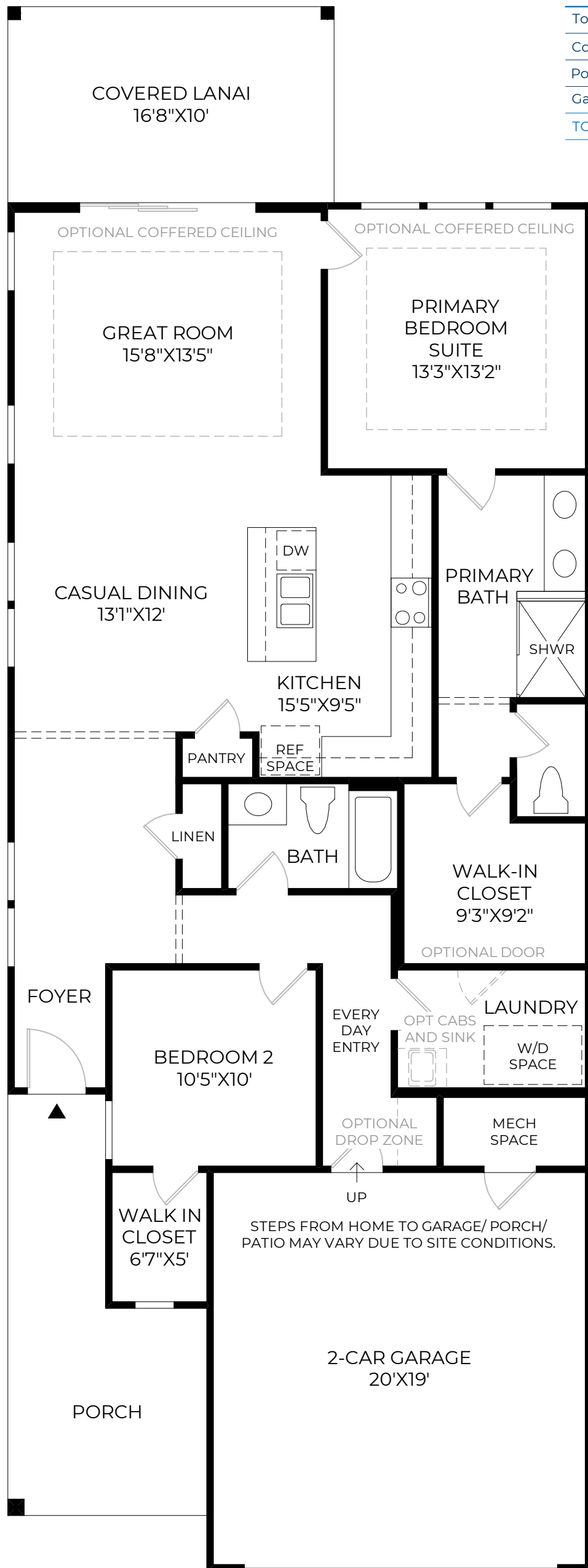
Floor Plan 9' CEILING HEIGHT
